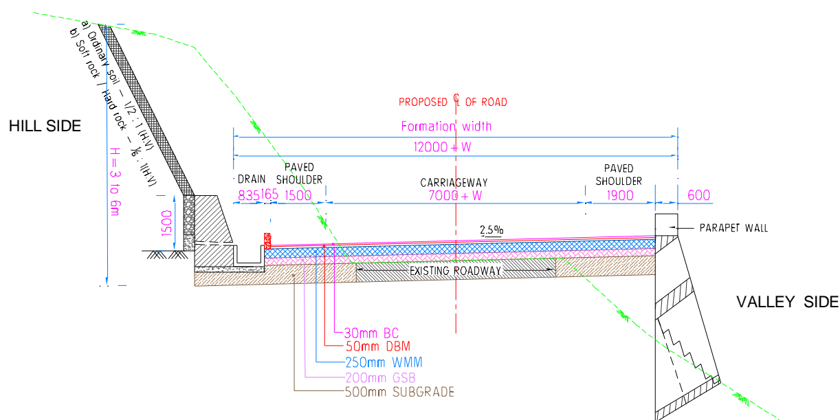
FIG. — 2B 2 — LANE CARRIAGEWAY WITH BREAST WALL OF 1.5M HEIGHT ON HILL SIDE AND RETAINING WALL ON VALLY SIDE — CONCENTRIC WIDENING (OPEN COUNTRY — MOUNTAINOUS TERRAIN)
