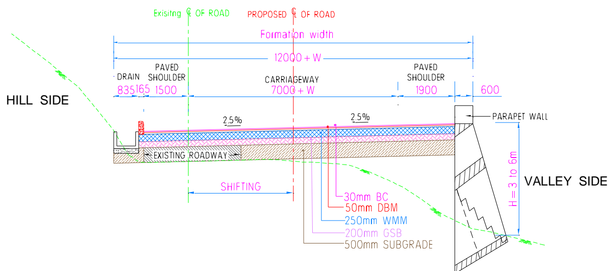
FIG. — 3A 2 — LANE CARRIAGEWAY WITH RETAINING WALL — VALLEY SIDE WIDENING (OPEN COUNTRY — MOUNTAINOUS TERRAIN)
