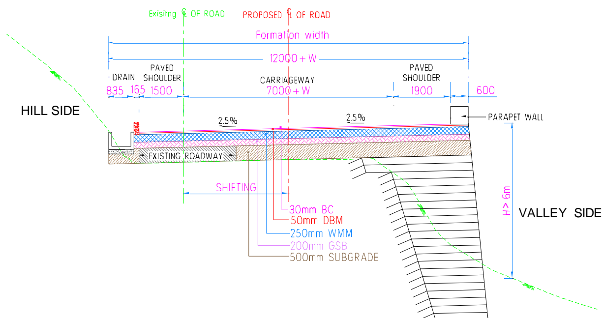
FIG. — 3B 2 — LANE CARRIAGEWAY WITH REINFORCED EARTH RETAINING WALL — VALLEY SIDE WIDENING (OPEN COUNTRY — MOUNTAINOUS TERRAIN)
