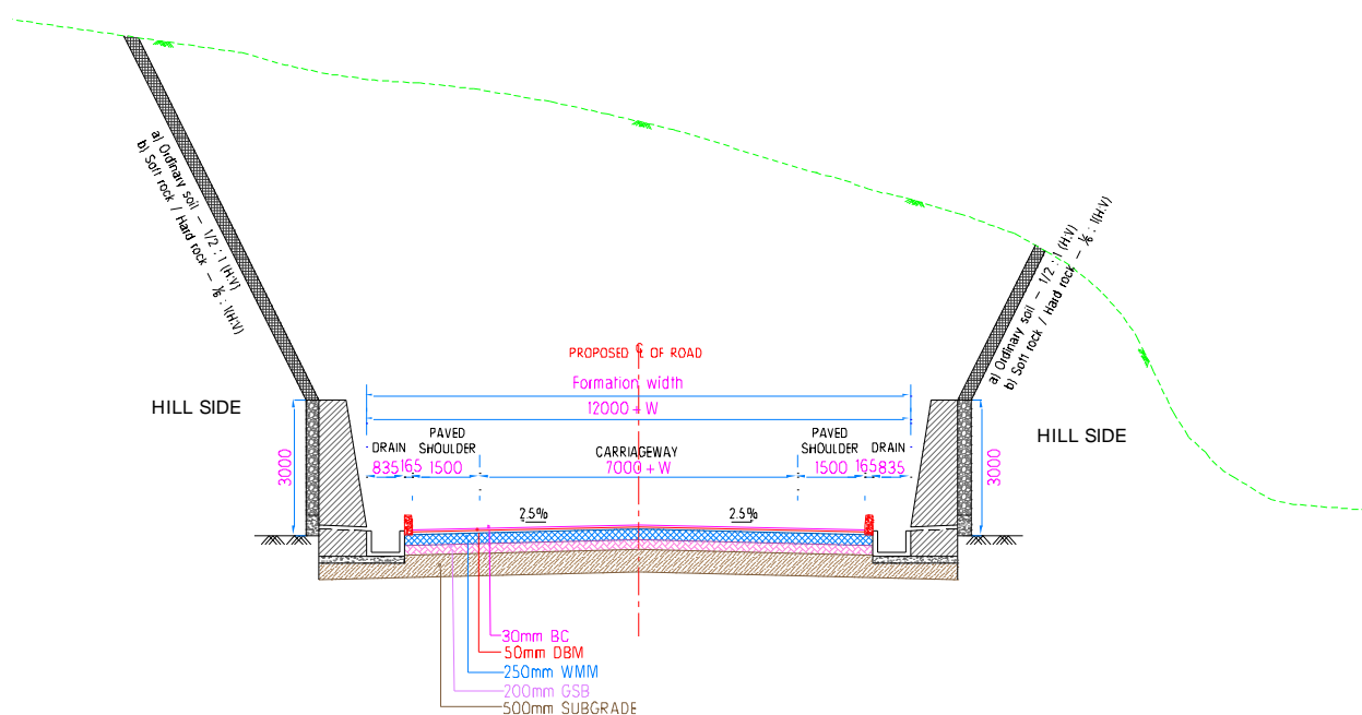
FIG. — 4 2 — LANE CARRIAGEWAY WITH BREAST WALL WITH BOX CUTTING — REALIGNMENT FROM HILL SIDE (OPEN COUNTRY — MOUNTAINOUS TERRAIN)
