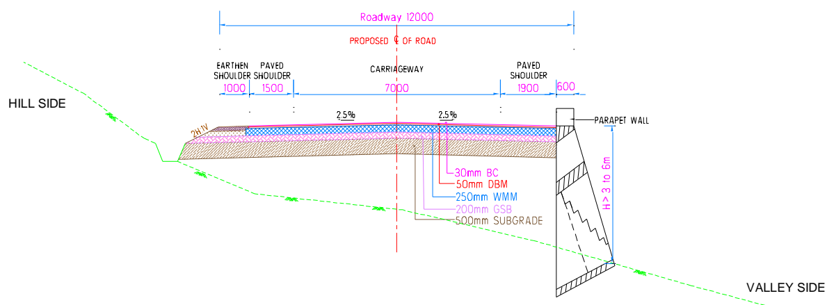
FIG. — 5A 2 — LANE CARRIAGEWAY WITH RETAINING WALL/REINFORCED EARTH RETAINING WALL — REALIGNMENT FROM VALLEY SIDE (OPEN COUNTRY — MOUNTAINOUS TERRAIN)
